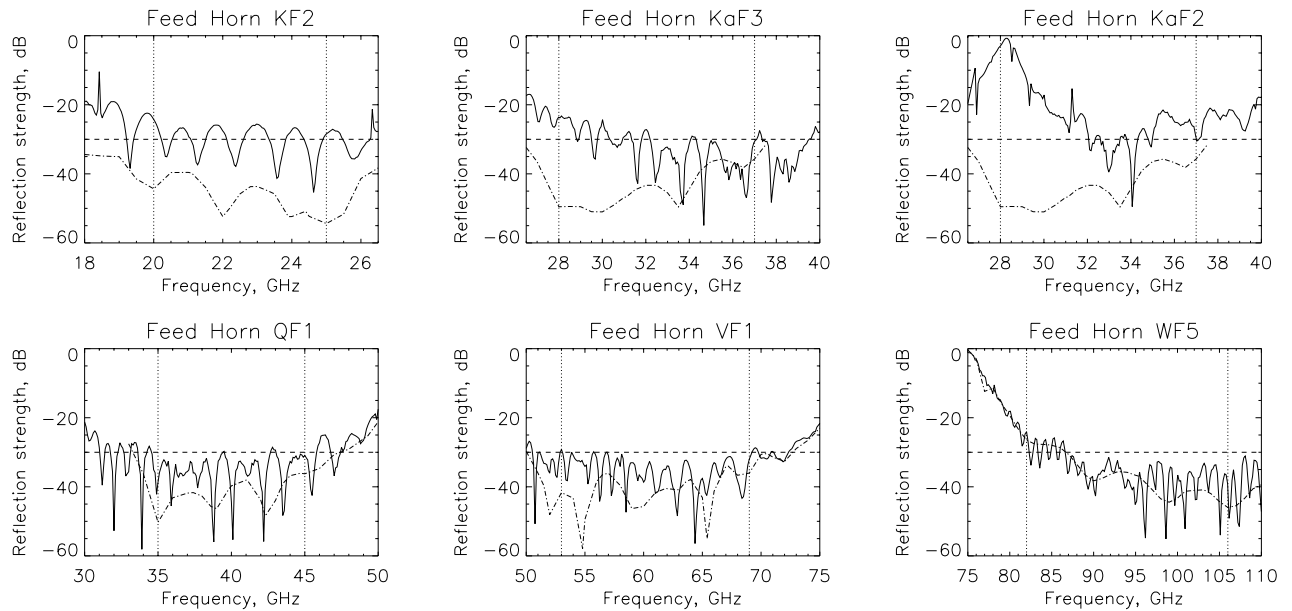
FIG. 7. — Predicted and measured reflected power for a selection of the MAP feed horns. The measured and predicted reflections are solid and dashed respectively. The reflected power is 10 \log_{10} |S_{11}|^2 where S is the scattering matrix. The vertical dotted lines mark MAP radiometer band edges, and the horizontal dashed line provides a reference at -30 dB. The measured reflection strengths show the combined effect of the rectangular-to-circular waveguide transition and the feed. (Predictions include only the feed.) In particular, the small regular oscillations in all the measured reflections correspond to the rectangular-to-circular transition length. In K band, the return loss is dominated by the transition; in W band it is dominated by feed. Feed KaF2 has a shallow spiral scratch inside its throat, an accident of fabrication. (KaF2 was not installed on the satellite.)
