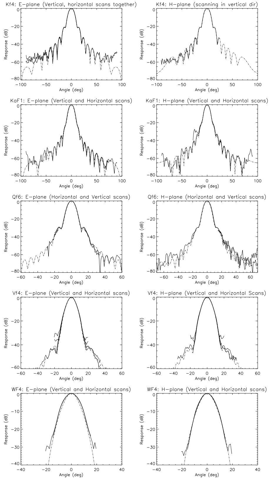
FIG. 5.— E and H-plane beam patterns for five feed horns. In these plots, the solid lines are measured responses and the dashed curves are predicted beam patterns, calculated as in section 4. With the exception of W-band, these beams were mapped in two stages: a first, inner map of the beam peak without an RF amplifier, and a second, outer map of the side-lobes with the amplifier installed. These measurements are matched at their overlaps. Each plot here overlays two scans: one vertical with the feed scanning from the sky (positive angles) down into the roof (negative angles), and one horizontal with the feed scanning from the source to the horizon at a cross elevation of about 80 deg. Discrepancies in the far side-lobes of these scans are evidence of reflections in the range. The little “legs” at -30 dB result from the noise floor of the main beam scan.
