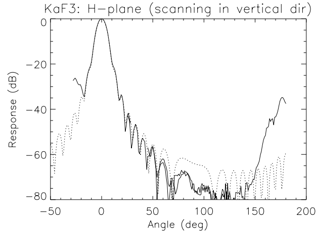
FIG. 6. — Two deep sidelobe measurements of a Ka band horn. Beyond 150 degrees, the horn looks below the horizon, and sees reflections from the ground. Below -25 degrees, another unwanted reflection dominates.
