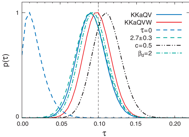
Figure 3. Distribution of the optical depth to reionization \tau for simulations with five-year WMAP noise levels. The optical depth is recovered for an individual simulation with \tau = 0.1 (black dashed line), for KKaQV and KKaQVW, and a \tau = 0 simulation is consistent with zero power. Changing the index priors to \beta_d = 2 , or \beta_s = -2.7 \pm 0.3 have negligible effects on the recovered CMB power. Incorrectly modeling the synchrotron as a power law for a simulation with an index that increases by c = 0.5 between 23 and 94 GHz increases \tau by \sim 1\sigma .
