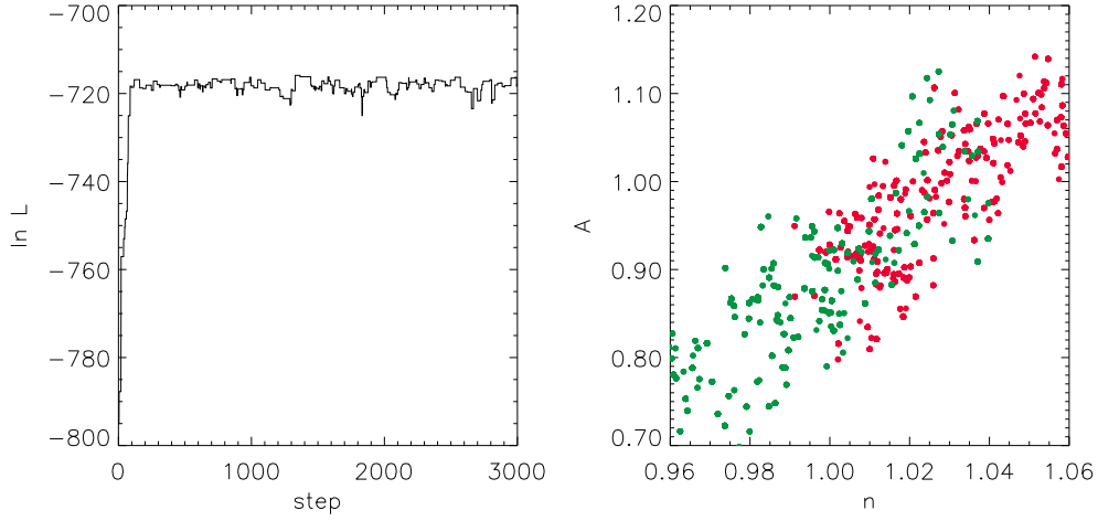
Fig. 3.— Unconverged Markov chains. The left panel shown a trace plot of the likelihood values versus iteration number for one MCMC (these are the first 3000 steps from one of our \Lambda CDM model runs). Note the burn-in for the first \sim 100 steps. In the right panel, red dots are points of the chain in the (n, A) plane after discarding the burn-in. Green dots are from another MCMC for the same data-set and the same model. It is clear that, although the trace plot may appear to indicate that the chain has converged, it has not fully explored the likelihood surface. Using either of these two chains at this stage will give incorrect results for the best fit cosmological parameters and their errors.
