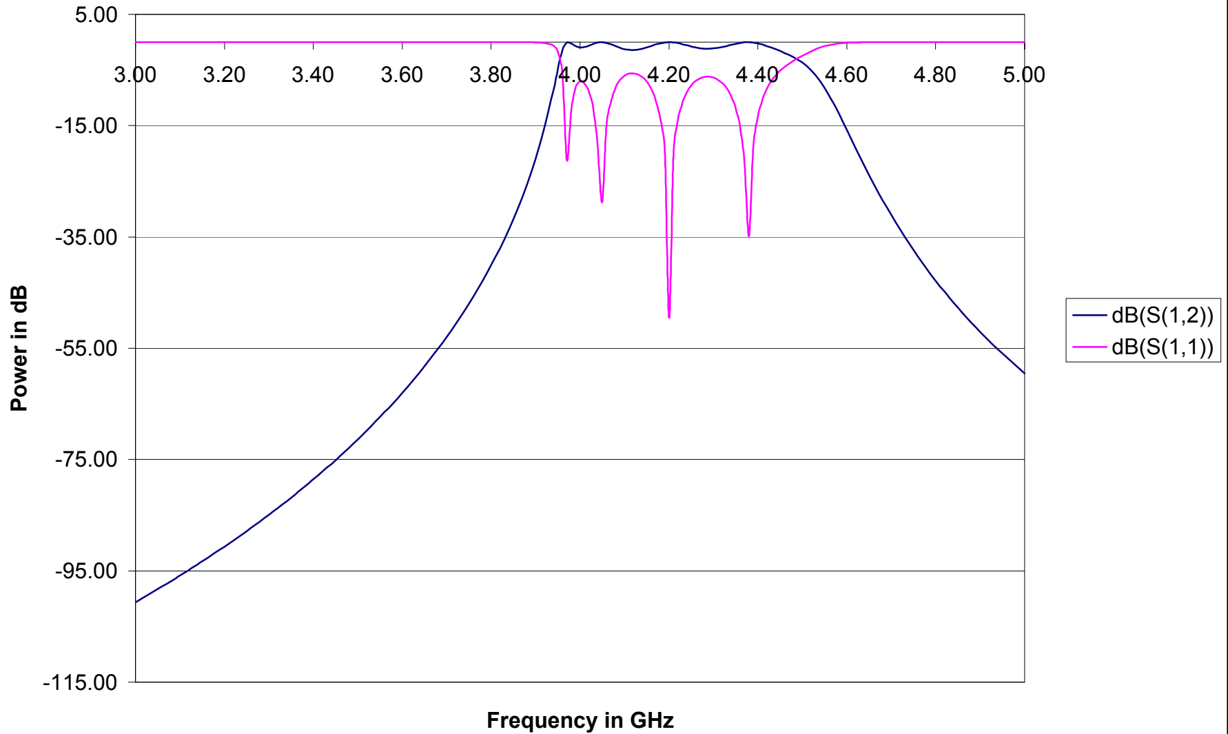
Linear Simulation Results for 4.25GHz Filter
