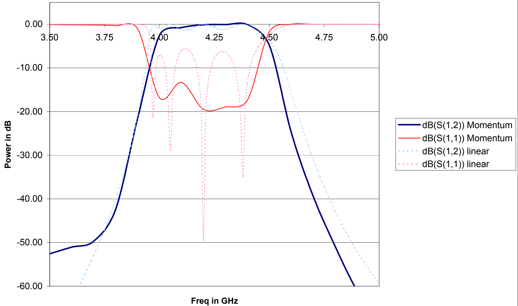
Mometum (full E&M) Simulation Results for 4.25GHz Filter
