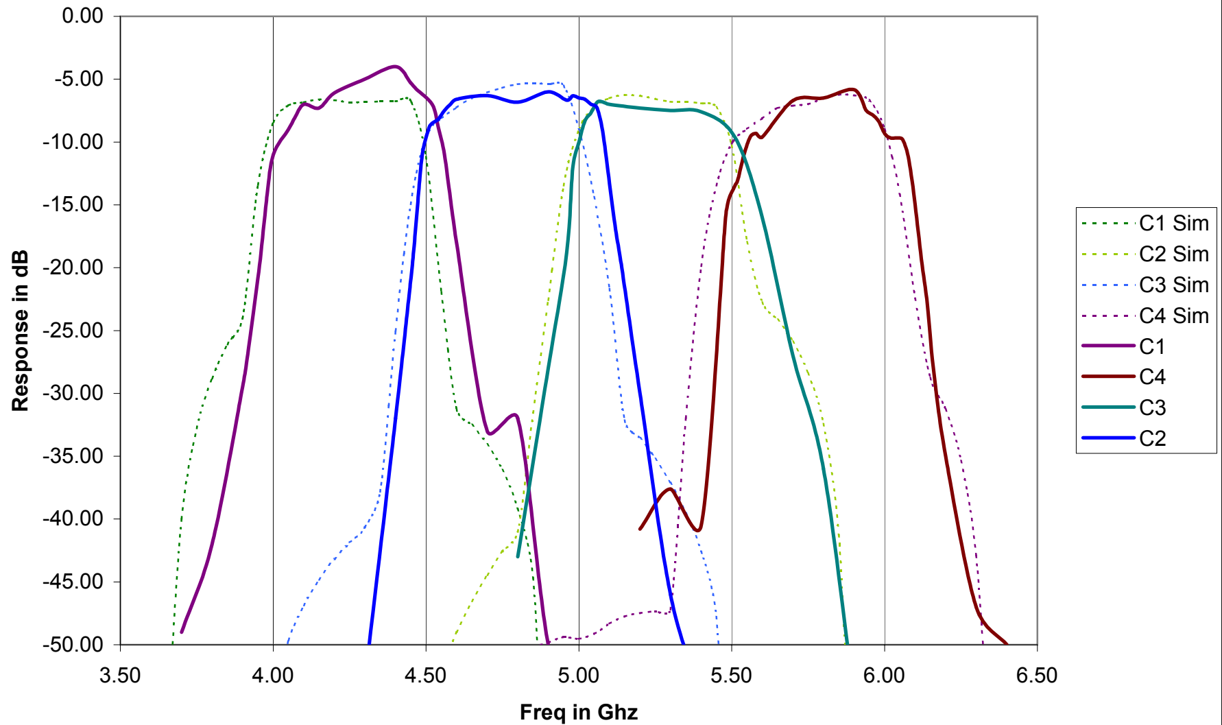
Channelizer performance with Mixers plotted with Simulations
