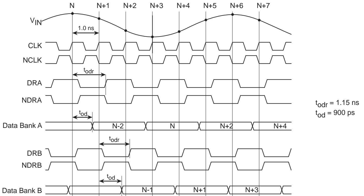
Figure 1 - Timing Diagram
