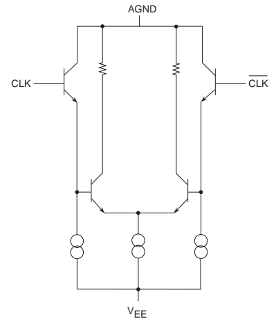
Figure 5C - Clock Input
