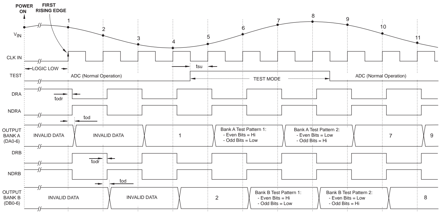
Figure 2 - Test Mode Timing Diagram
