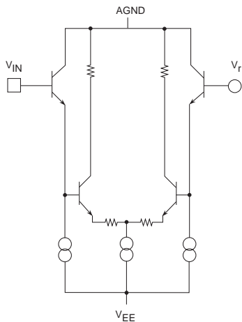
Figure 4A - Input Circuit
