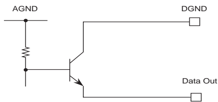
Figure 4B - Output Circuit
