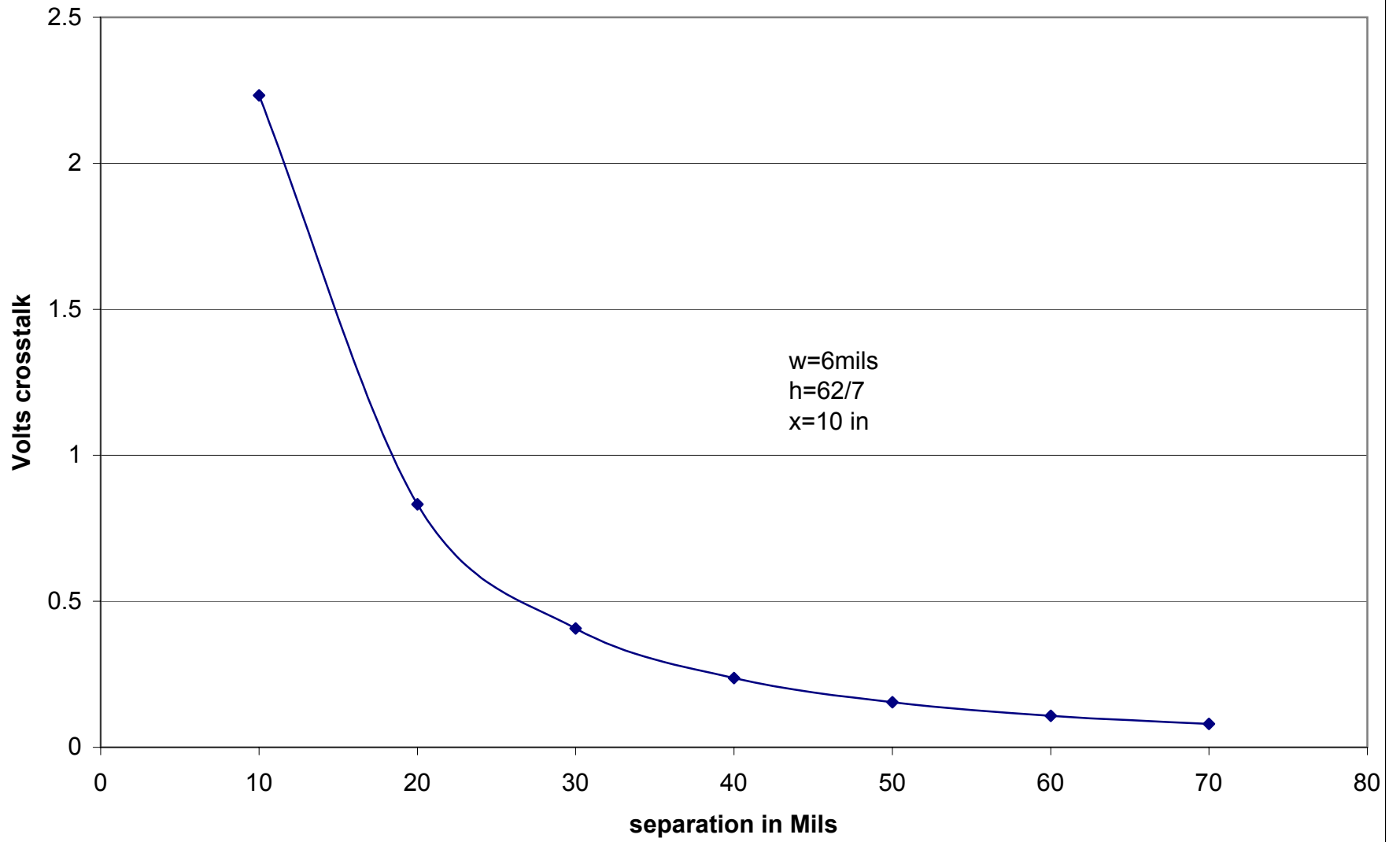
Crosstalk @ 3.3V and 1ns rise time
