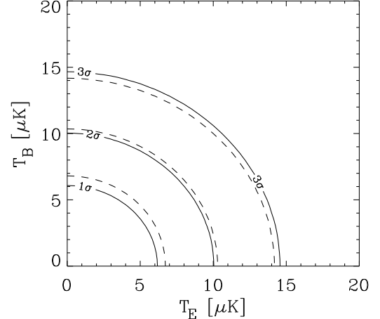
FIG. 2.— Normalized likelihood contour plots in the T_E - T_B plane. The contours enclose 68%, 95.4%, and 99.7% of the total probability, corresponding to 1, 2, and 3 standard deviation intervals, as labeled. The solid lines correspond to the joint likelihood for the combined three frequency channels, and the dashed lines are the corresponding null-channel (QPC) likelihood.
