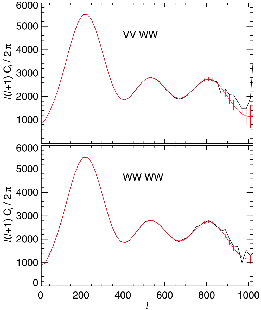
Fig. 13.— The quadratic estimator discussed in §A.1 has been extensively tested with Monte Carlo simulations of first-year WMAP data. The top panel shows a model spectrum in red, and the mean of 600 realizations of the cross-power spectrum, computed from the V and W band-averaged maps, in black. The red error bars show the uncertainty in the mean in bins with \Delta l = 20 . The cross-power spectrum estimator is unbiased. The bottom panel is similar, but with auto-power spectra computed from the W band-averaged map. Here the noise bias term was estimated directly from the high l tail of the computed spectrum. This simple auto-power spectrum estimator is unbiased if the noise is white, and is suitable for V band data, but see Figure 1 for examples of W band noise spectra.
