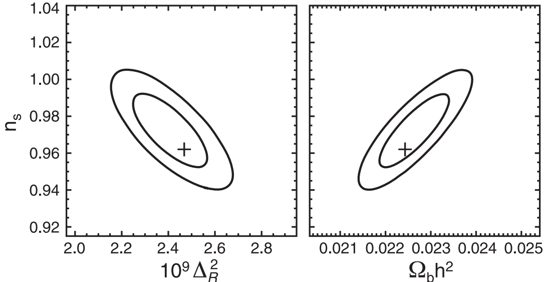
FIG. 3.— 68% and 95% CL regions for the \Lambda CDM parameters n_s , 10^9 \Delta_{\mathcal{R}}^2 , and \Omega_b h^2 . There is a modest degeneracy between these three parameters in the six-parameter \Lambda CDM model, when fit to the nine-year WMAP data. The contours are derived from fits to the C^{-1} -weighted power spectrum, while the plus signs indicate the maximum likelihood point for the fit to the MASTER power spectrum. As shown in Figure 2, the two model produce nearly identical spectra.
